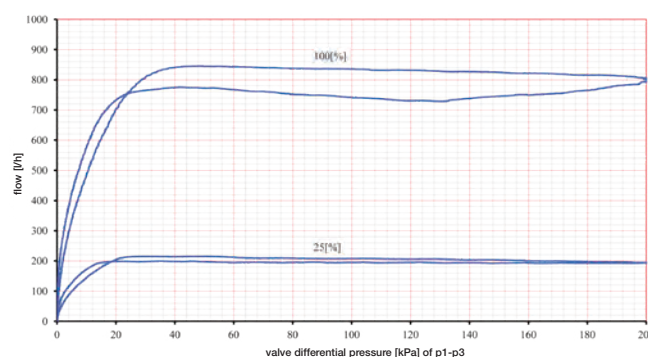
Hysteresis for 25% and 100% flow for the flow controller 4001
