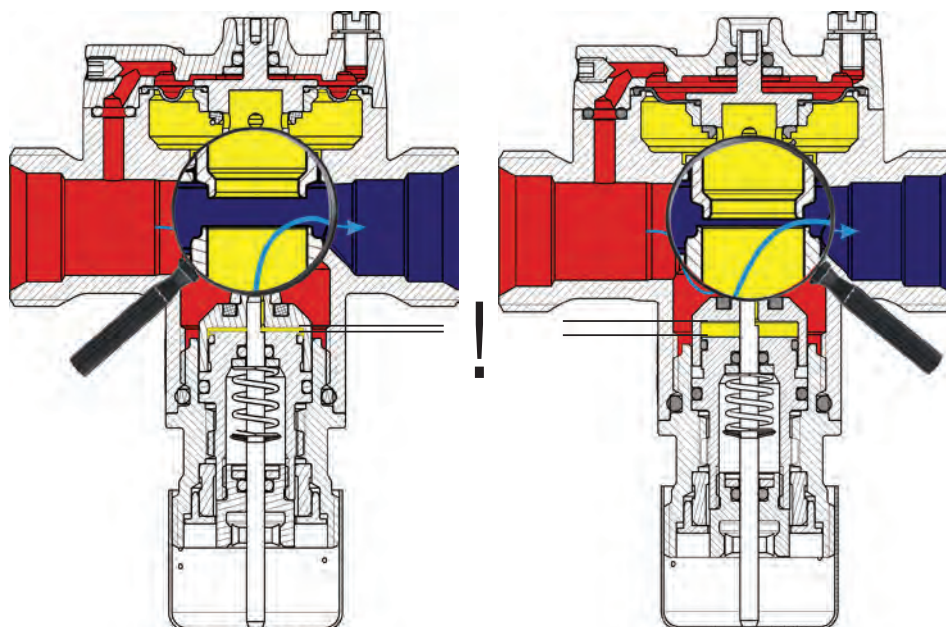
HERZ 4006 SMART in fully open position
